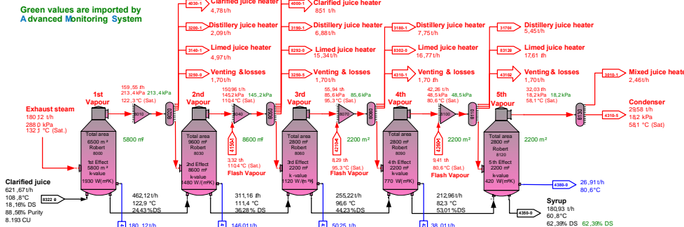
Figure 2: Simulation model of an evaporation station
