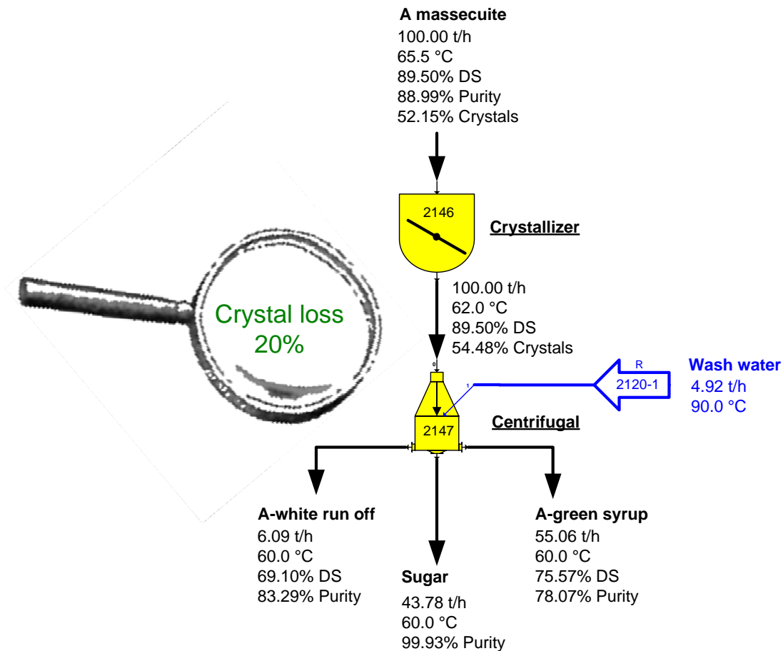
Figure 3: Excerpt from a sugar house simulation model
